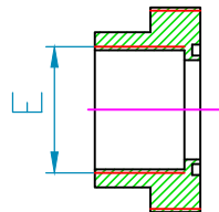
FEMALE PIPE THREAD
