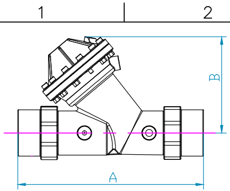
FEMALE SOCKET WELD END CONNECTORS
