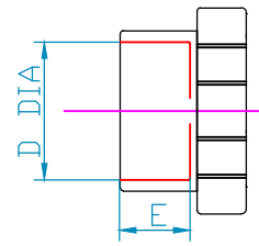
FEMALE SOCKET WELD END CONNECTORS
